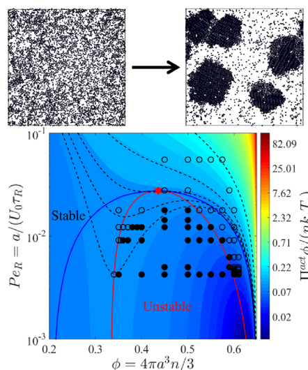
Figure : Athermal phase separation of active matter. (Adapted from Takatori & Brady, PRE (2015))
